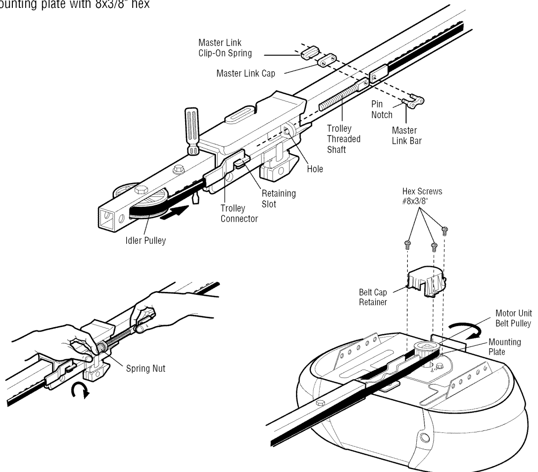
Spring/Trolley Nut
