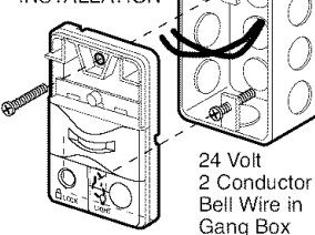
Figure 2 PRE WIRED INSTALLATION
