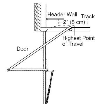
One-piece door with horizontal track
