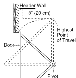
One-piece door without track: pivot hardware
