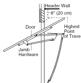
One-piece door without track: jamb hardware
