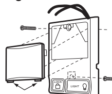
Figure 1 INSTALLATION STANDARD
