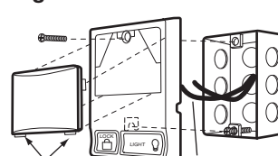
Figure 2 INSTALLATION PRÉ-CABLÉE
